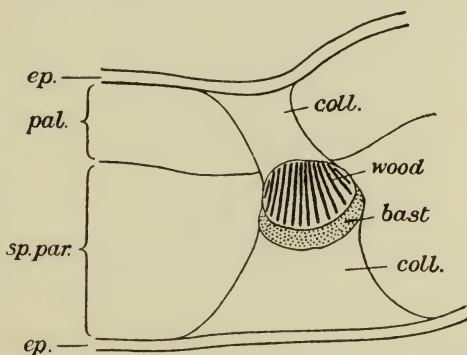
FIG. 53.—Bearberry Leaf. Diagrammatic section of midrib, showing the distribution of the various tissues. \times 65 .
